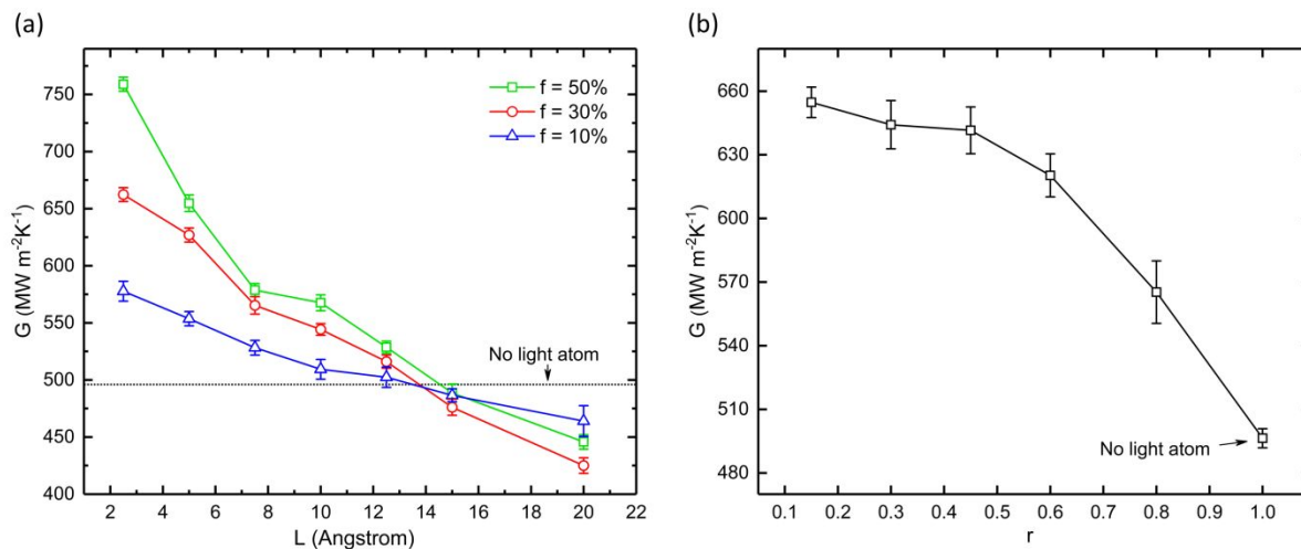
Fig. 2 (a) G_{SiC/GaN} ( r = 0.15 , light atom has the mass of boron) as a function of the skin depth ( L ) of the doped region with different concentrations, where Ga are randomly substituted with light atoms. (b) G_{SiC/GaN} by varying r , the ratio of the light atom mass over the mass of Ga, with L = 5 \text{ \AA} .
