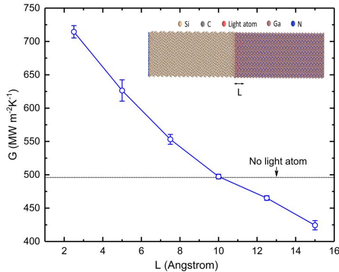
Fig. 3 G_{SiC/GaN} as a function of L with f = 10\% when boron atoms ( r = 0.15 ) are incorporated into the GaN layer as interstitial additives. The inset is a schematic of the structure.
